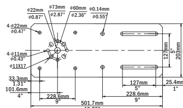
WASHER PLATE (T=7mm)
