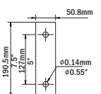
WASHER PLATE (T=7mm)
