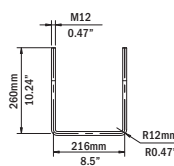
U-BOLT (QTY: 2)
